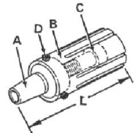
Standard Length Adjustable Depth Chuck Type 4
