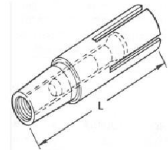
Standard Length Adjustable Depth Chuck Type 3
